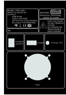
Back panel
